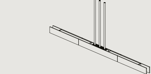
LP:1390.TD L1390 W48 H64 / L54.7" W1.9" H2.5" MIN DROP HEIGHT - H300 / 11.8"
