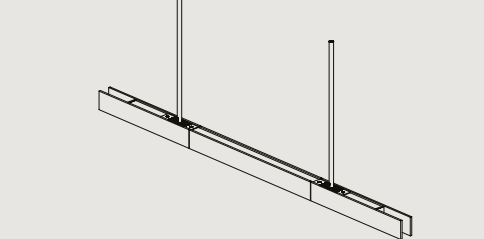
LP:1390.DD L1390 W48 H64 / L54.7" W1.9" H2.5" MIN DROP HEIGHT - H300 / 11.8"
