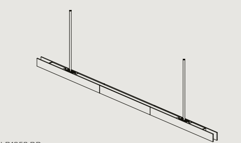
LP:1950.DD L1950 W48 H64 / L76.8" W1.9" H2.5" MIN DROP HEIGHT - H300 / 11.8"
