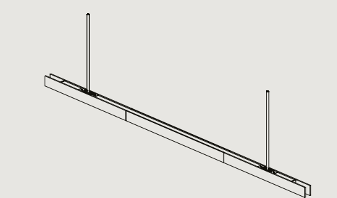
LP:2230.DD L2230 W48 H64 / L87.8" W1.9" H2.5" MIN DROP HEIGHT - H300 / 11.8"
