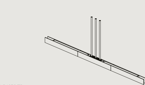
LP:1670.TD L1670 W48 H64 / L65.7" W1.9" H2.5" MIN DROP HEIGHT - H300 / 11.8"
