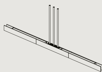
LP.1670.TD L1670 W48 H64 / L65.7" W1.9" H2.5" MIN DROP HEIGHT - H300 / 11.8"
