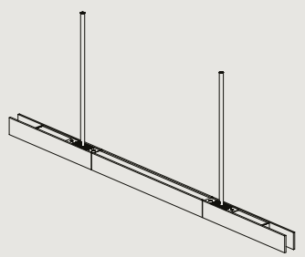
LP.1390.DD L1390 W48 H64 / L54.7" W1.9" H2.5" MIN DROP HEIGHT - H300 / 11.8" CEILING CANOPY SPACING - 700MM / 27.56"
