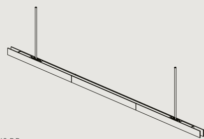
LP.2510.DD L2510 W48 H64 / L98.8" W1.9" H2.5" MIN DROP HEIGHT - H300 / 11.8" CEILING CANOPY SPACING - 1820MM / 71.65"
