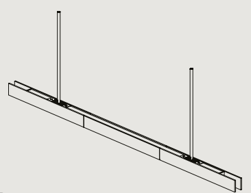
LP.1670.DD L1670 W48 H64 / L65.7" W1.9" H2.5" MIN DROP HEIGHT - H300 / 11.8" CEILING CANOPY SPACING - 980MM / 38.58"
