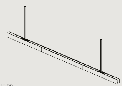
LP.2230.DD L2230 W48 H64 / L87.8" W1.9" H2.5" MIN DROP HEIGHT - H300 / 11.8" CEILING CANOPY SPACING - 1540MM / 60.63"
