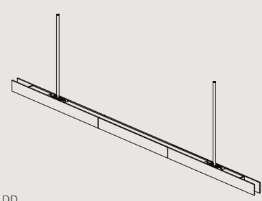
LP.1950.DD L1950 W48 H64 / L76.8" W1.9" H2.5" MIN DROP HEIGHT - H300 / 11.8" CEILING CANOPY SPACING - 1260MM / 49.61"
