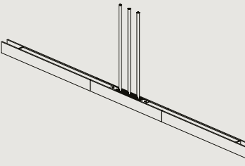
LP.1950.TD L1950 W48 H64 / L76.8" W1.9" H2.5" MIN DROP HEIGHT - H300 / 11.8"
