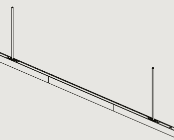
LP.2510.DD L2510 W48 H64 / L98.8" W1.9" H2.5" MIN DROP HEIGHT - H300 / 11.8" CEILING CANOPY SPACING - 1820MM / 71.65"
