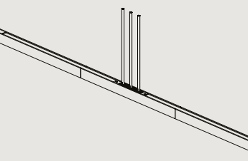
LP.2510.TD L2510 W48 H64 / L98.8" W1.9" H2.5" MIN DROP HEIGHT - H300 / 11.8"
