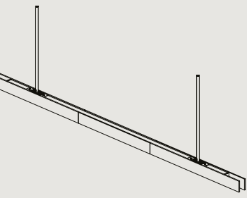
LP.1950.DD L1950 W48 H64 / L76.8" W1.9" H2.5" MIN DROP HEIGHT - H300 / 11.8" CEILING CANOPY SPACING - 1260MM / 49.61"
