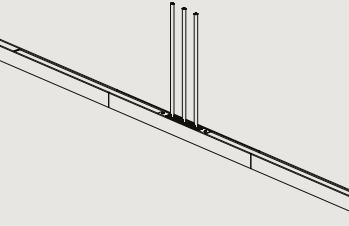
LP.2230.TD L2230 W48 H64 / L87.8" W1.9" H2.5" MIN DROP HEIGHT - H300 / 11.8"
