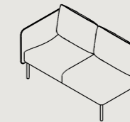
ASA2-R/L* W 1410 D 730 H 815 S 440
