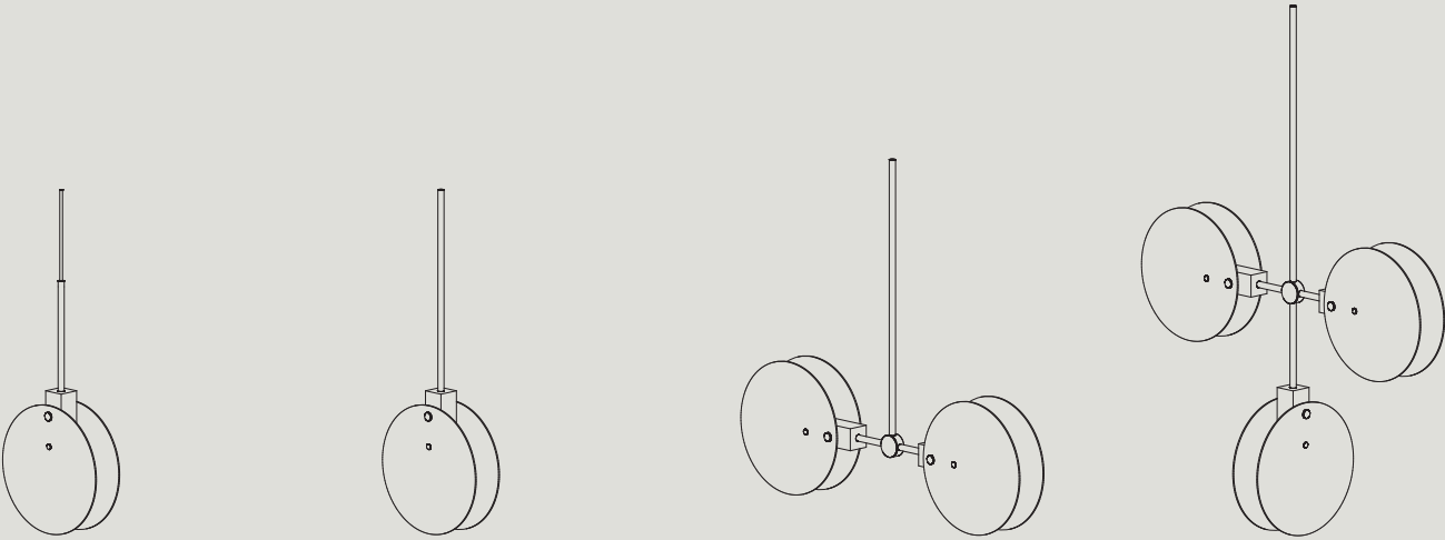
NC11 CORDED L 300 W 87 H 590 L 11.8" W 3.4" H 23.2" NC11 TUBE L 300 W 87 H 330* L 11.8" W 3.4" H 13.0"** NC12 L 870 W 87 H 300* L 34.3" W 3.4" H 11.8"** NC13 L 870 W 300 H 696* L 34.3" W 11.8" H 27.4"**
