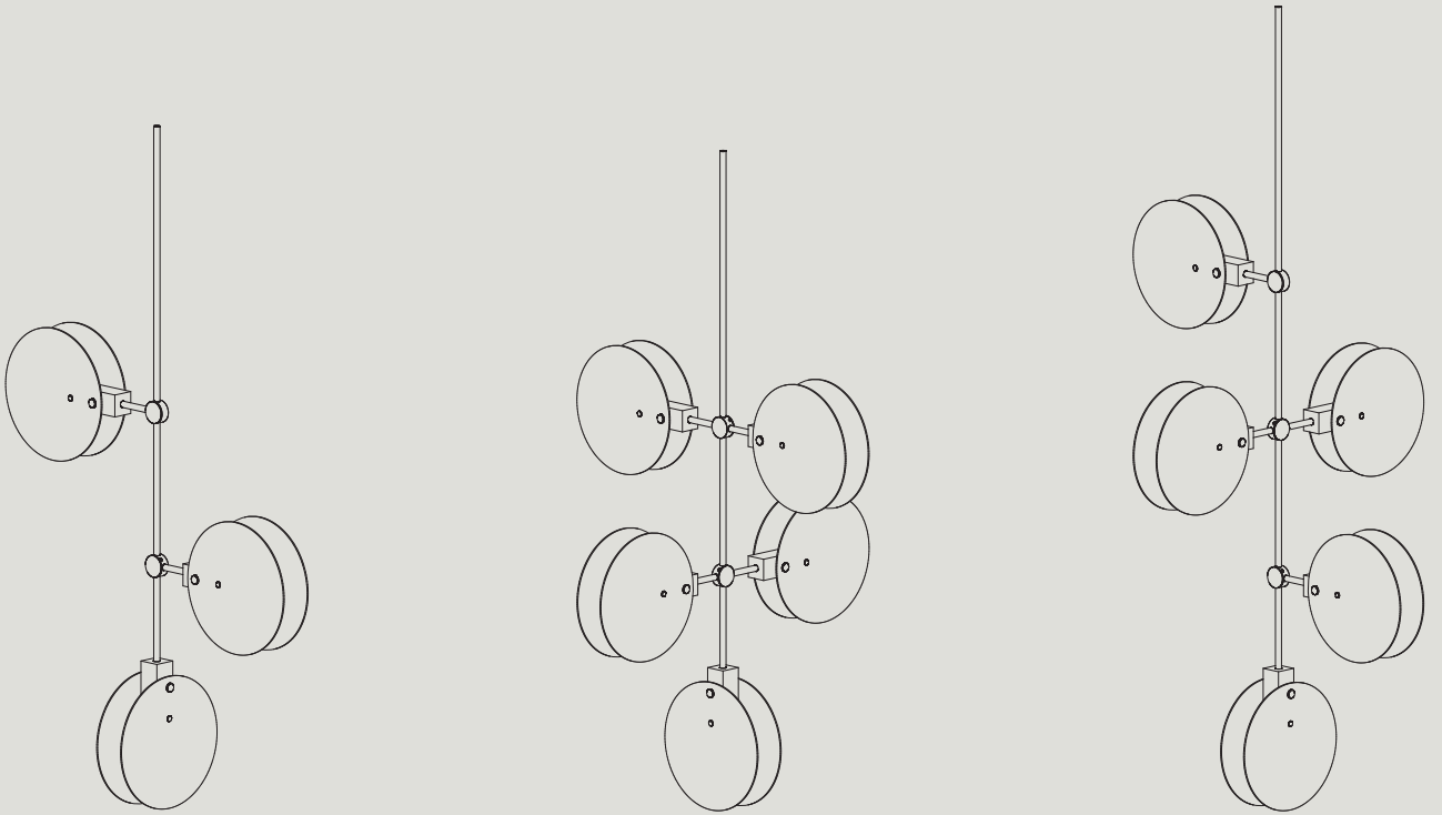
NC13 OFFSET L 870 W 300 H 1046* L 34.3" W 11.8" H 41.2"** NC15 L 870 W 870 H 1046* L 34.3" W 34.3" H 41.2"** NC15 OFFSET L 870 W 870 H 1396* L 34.3" W 34.3" H 55.0"**
