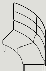
AHB2-S# W 1360 D 730 H 1350 S 440
