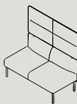
AHB2-S# W 1360 D 730 H 1350 S 440
