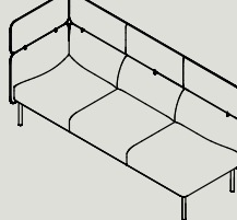
AMA3-R/L* W 2090 D 730 H 1025 S 440
