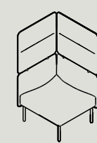
AHC1-S-R/L*#^ W 730 D 730 H 1350 S 440
