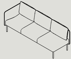
ASA3-R/L* W 2090 D 730 H 815 S 440 W 82.3" D 28.7" H32.1" S17.3"
