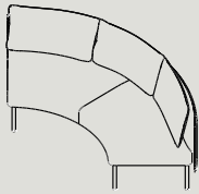
ASB90 W 1530 D 1530 H 815 S 440 IN Ø1600 / OUT Ø3,040 W 60.2" D 60.2" H32.1" S17.3" IN Ø63.0" / OUT Ø119.7"
