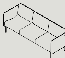
ASL3 W 2140 D 730 H 815 S 440 W 84.25" D 28.7" H32.1" S17.3"
