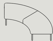
ASO90 W 1480 D 1480 H 440 IN Ø1600 / OUT Ø2,960 W 58.3" D 58.3" H 17.3" IN Ø63.0" / OUT Ø116.5"
