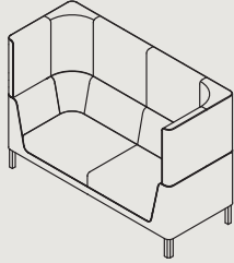
TWO SEATER HIGH-BACK W 1900 D 770 H 1300 S 400
