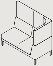
TWO SEATER SINGLE ARM HIGH-BACK W 1530 D 770 H 1300 S 400
