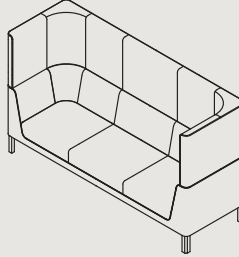
THREE SEATER HIGH-BACK W 2300 D 770 H 1300 S 400
